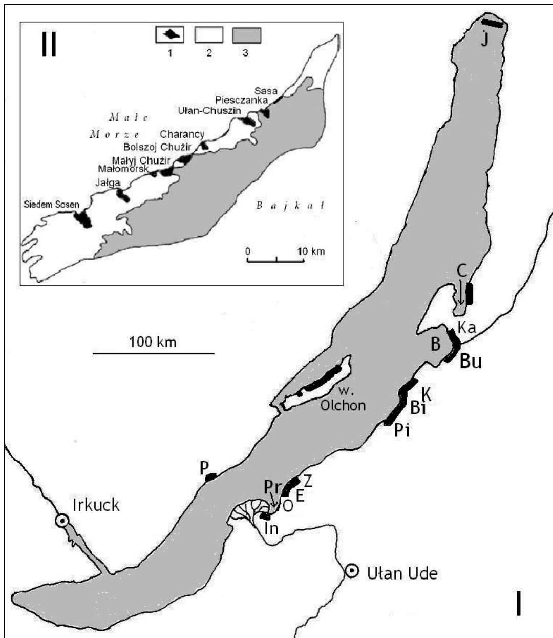
Fig. 1. The location of the main fields of blown-out sands on the coast of Lake Baikal (I) and a gentle shore of Olkhon (II): I: B – Barguzin Bay, C – Chivyrkuy Bay, P – Sandy (Peschanaya) Bay, Pr – Proval Bay, J – Yarki island; dune sites: Bi – Bezmyannaya, Bu – Bugry, E – Enkheluk, In – Inkino, K – Katkova, Ka – Karga, O – Oblom, P – Peschanoye, Z – Zagza; II: sites of contemporary aeolian sands, 2 – steppe areas, 3 – taiga areas
